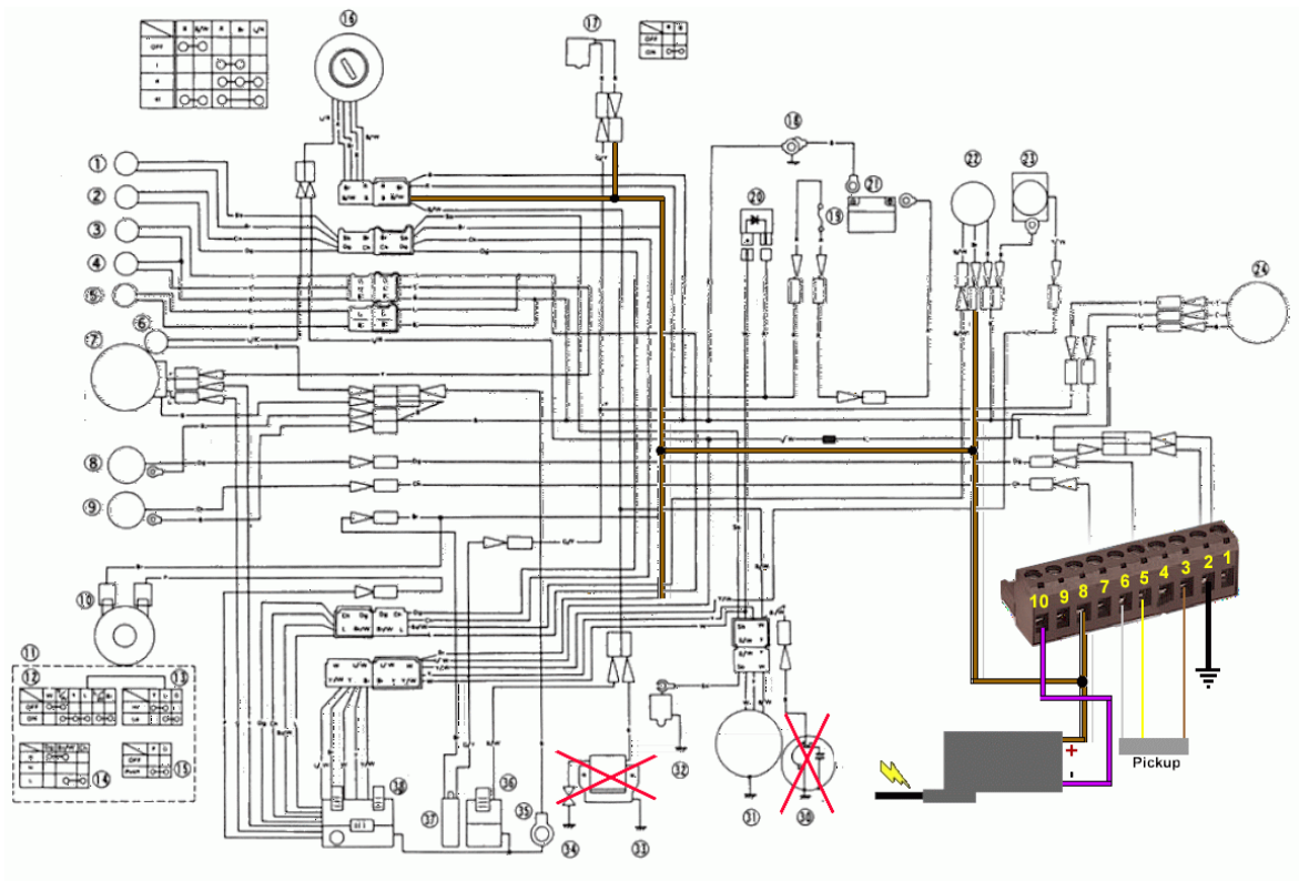
Ignition circuit diagram
